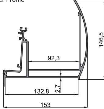
10-10093 Duvar Profili / Wall Profile 1.942 kg/m
