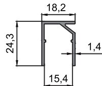
10-10091 Polikarbon Kapama Çıtasa Profili/Polycarbonate Cover Strip Profile 0.252 kg/m
